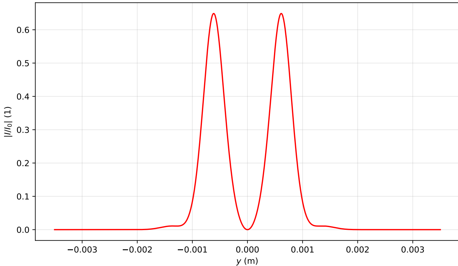
Intensity profile I(x=0, y, z=1.115)/I_0 , P_{in}=4.0P_{cr} , artificial time
